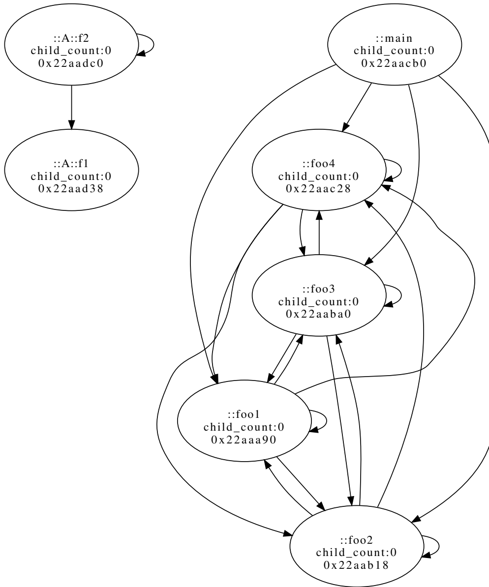
Figure 24.3: Call graph for function in input code file: inputCode.BuildCG.C.
