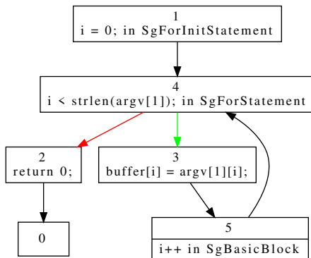
Figure 21.3: Control flow graph for function in input code file: inputCode_1.C.
